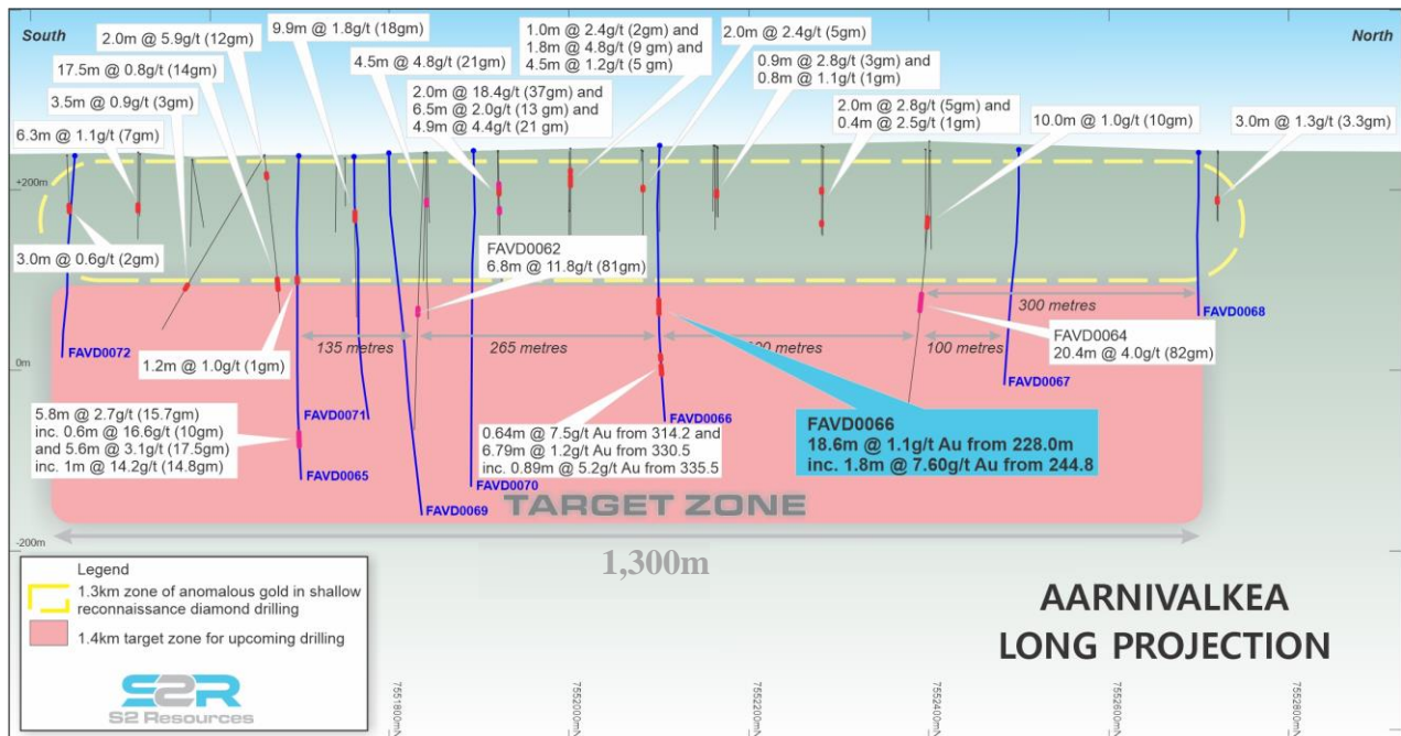
Figure 2. Long projection of the Aarnivalkea prospect showing recently completed holes, the target zone for the ongoing drilling program and selected intercepts from previous diamond drilling.
