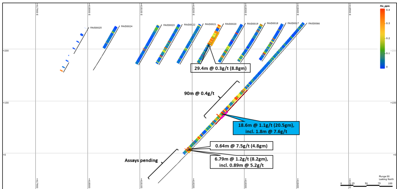
Figure 1. Cross section showing gold mineralisation in hole FAVD0066, including the recent intercept (blue) and previously reported intercepts (white)
