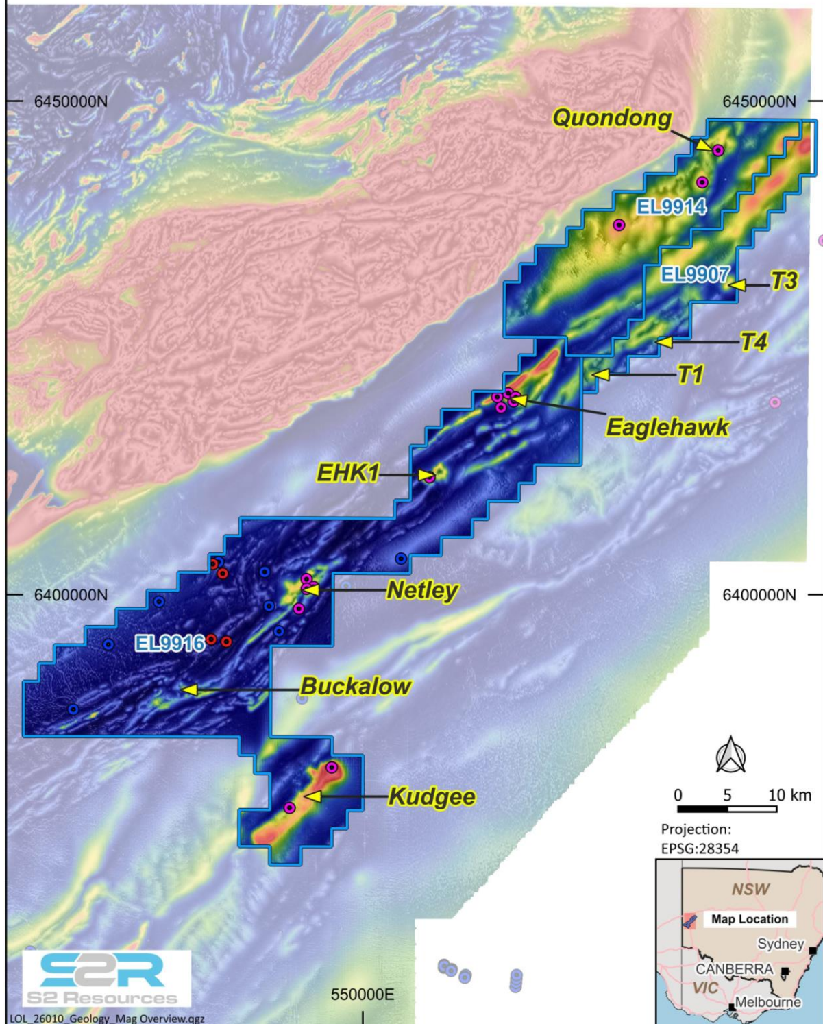
Figure 3. Magnetic image showing Eaglehawk and Netley prospects, and other porphyry targets.
