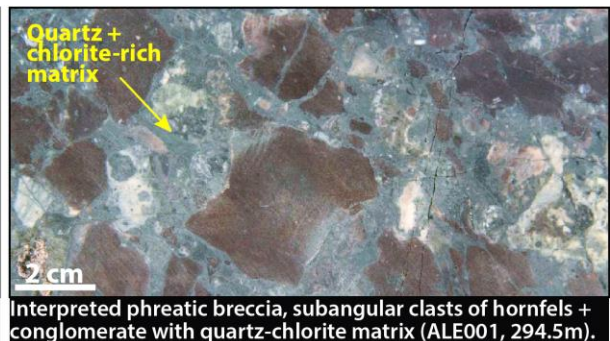
Figure 5. Alteration and host rock examples from the Eaglehawk prospect (ALE001). Core photos and interpretations are re-produced from open file and internal company reports 5,6,7,8 .
