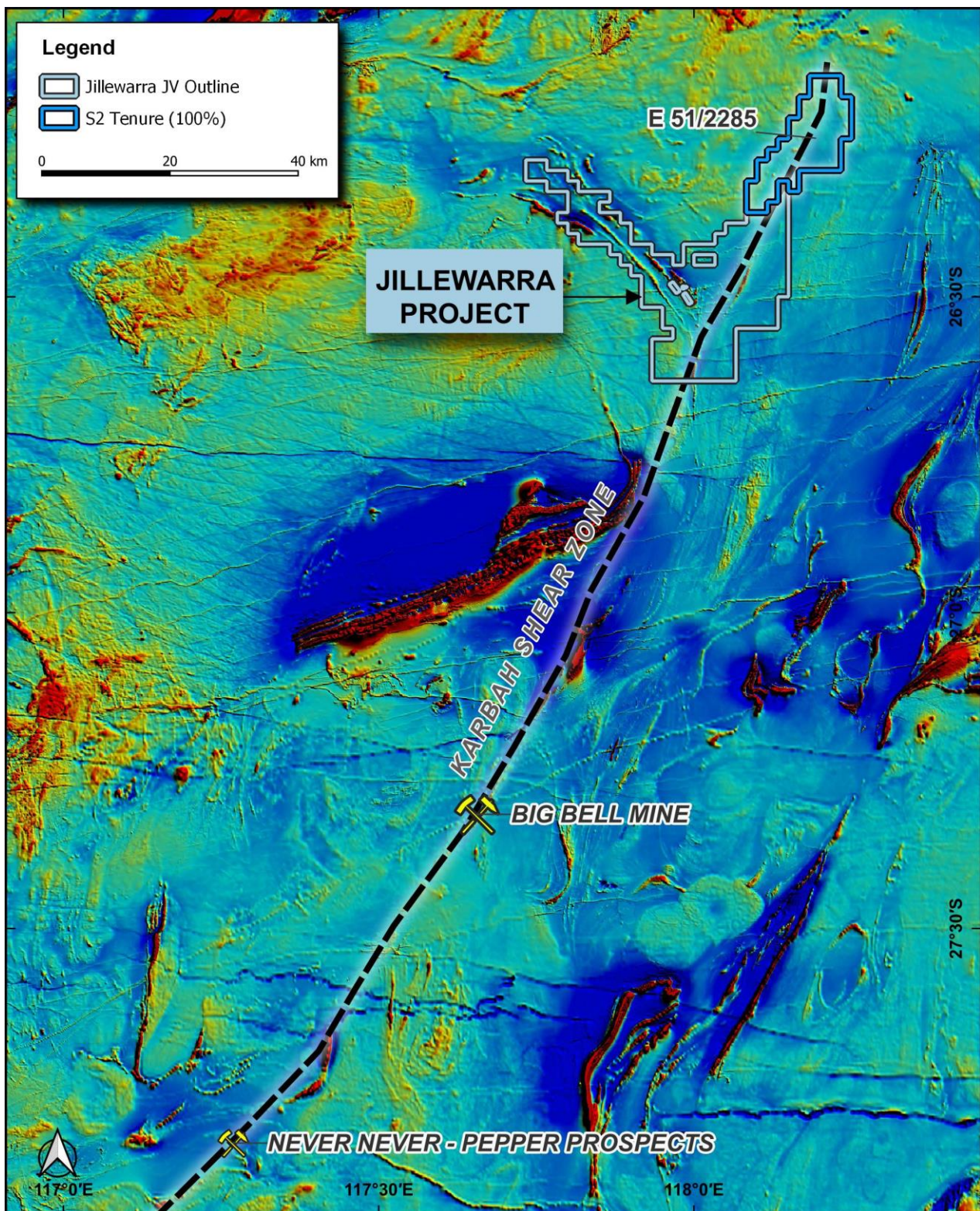
Figure 5. Regional aeromagnetic image of Murchison district showing the new outline of the Jillewarra project covering the interpreted regional shear zone that extends south through Westgold's Big Bell gold mine and Spartan Resources' recent discoveries at their Dalgara project (the Never Never and Pepper gold deposits).
