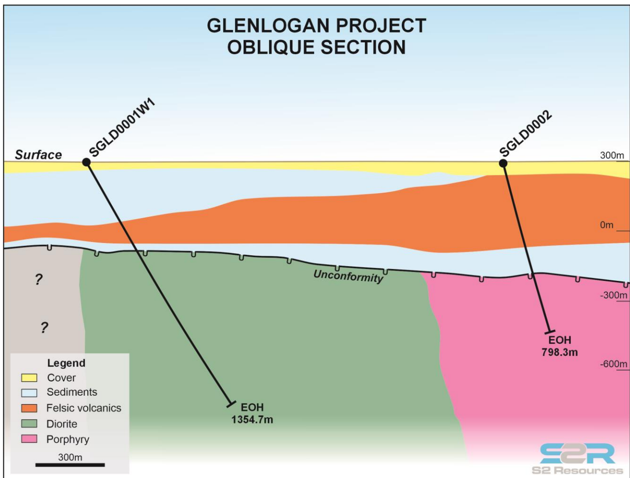
Figure 9. Oblique cross section showing position of holes SGLD001W1 and SGLD0002, with generalised geology.
